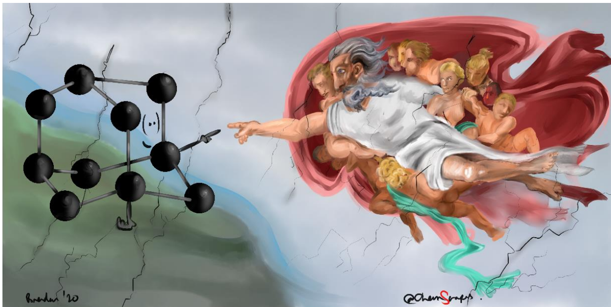
The Creation of Adamantane, 2020. @ChemScrapes SciArt collection.
